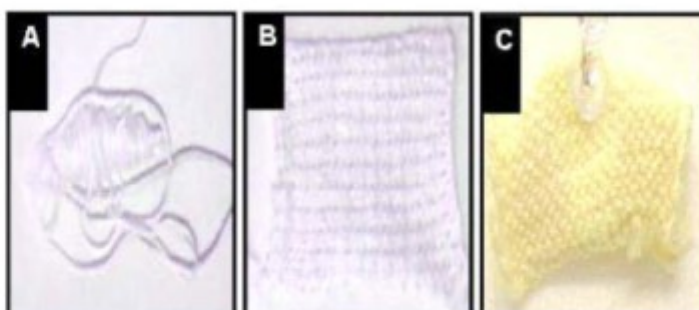
Figure 3.5 From left to right: A cotton thread coated with the NRL enzyme catalytic system (A) and woven into a piece of textile fabric (B). Following contact with a pesticide solution, the textile takes on a yellowish colour (C) that is characteristic of the completed neutralization process (source: Naval Research Laboratory)
